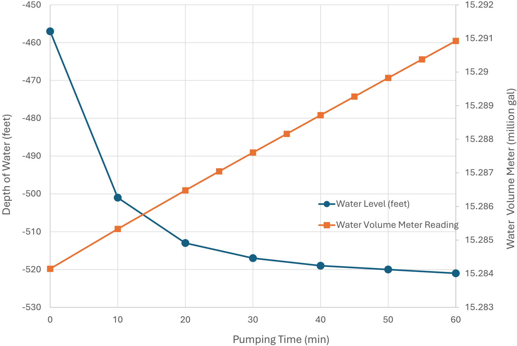
Drawdown Test 15Apr2024
